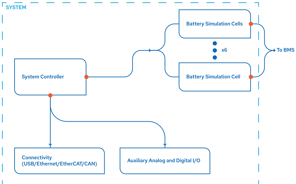
Figure 1: Block Diagram of DE3011
