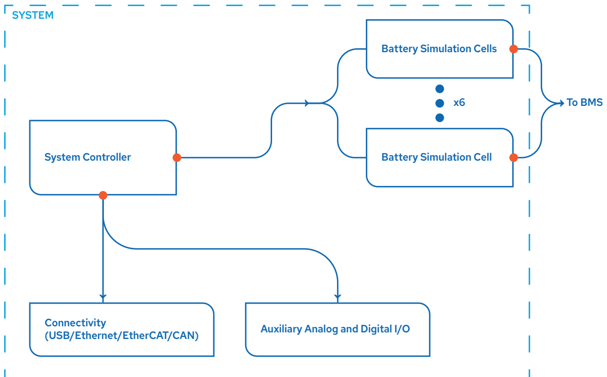
Figure 1: Block Diagram of DE3001
