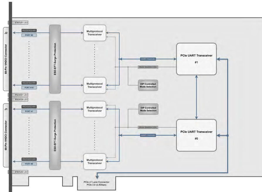
Figure 1: Block Diagram of DE180500
