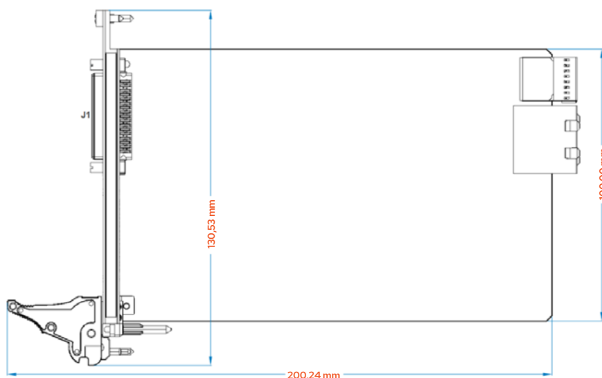
Figure 2: Module Dimensions
