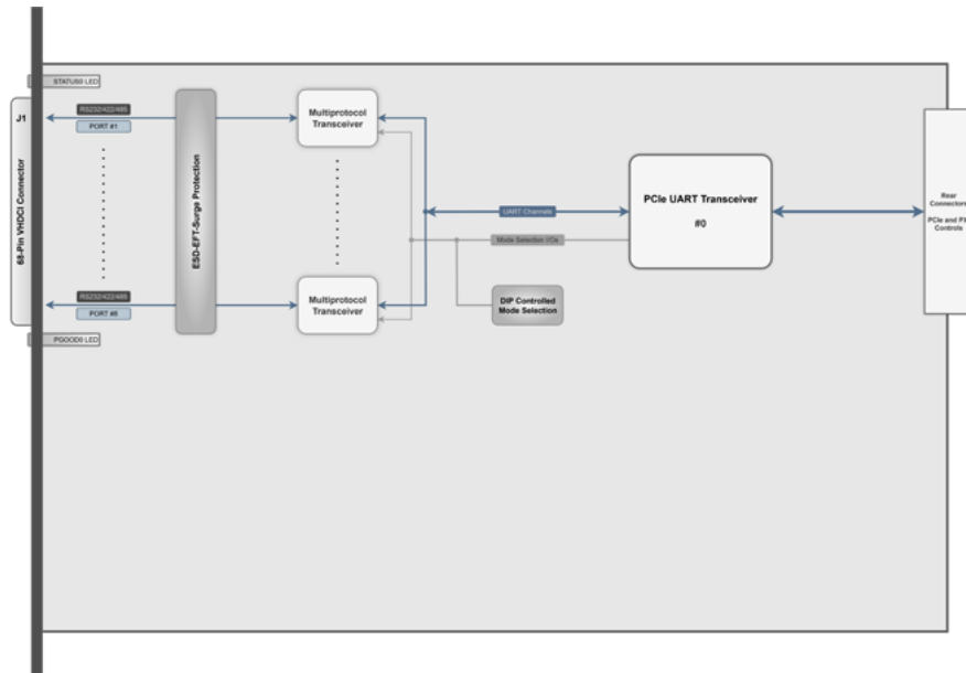
Figure 1: Block Diagram of DE140501
